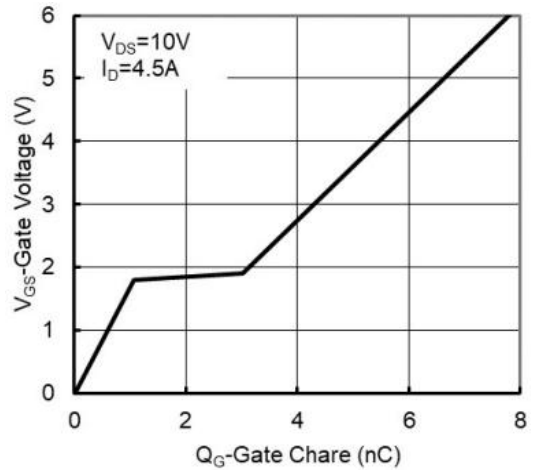
Figure 6: Gate-Charge Characteristics
