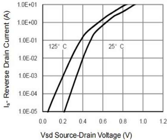
Figure 7: Diode Characteristics
