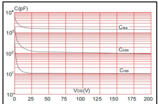
Figure 6: Capacitance Characteristics
