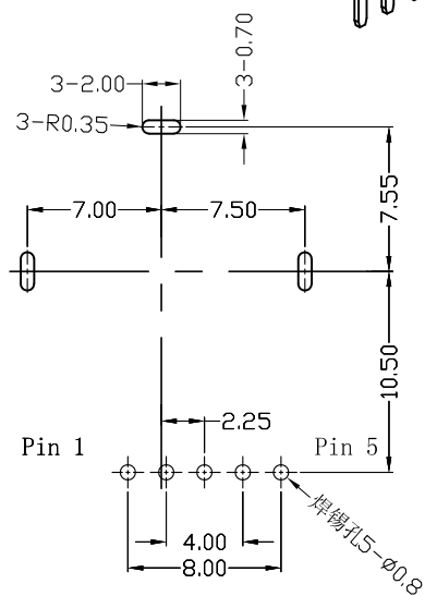
P. C. B MOUNTING HOLE DETAIL
