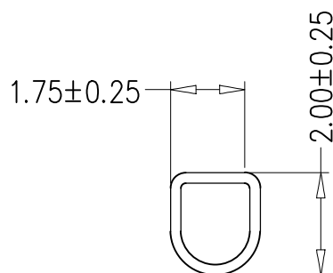
SEC: C-C
