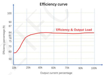
Figure : Efficiency VS Output Load (Nominal Voltage Input)
