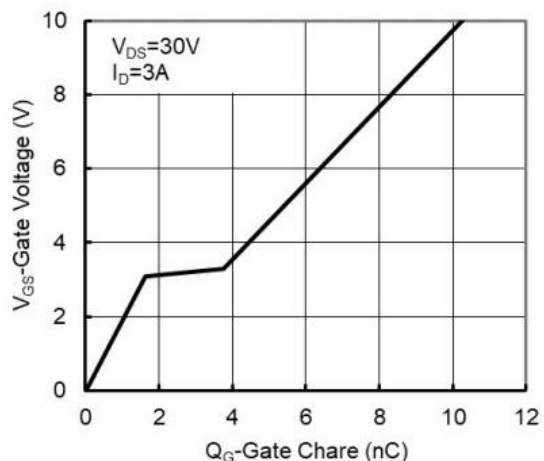
Figure 6: Gate-Charge Characteristics
