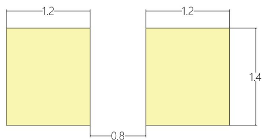
建议焊盘尺寸 Recommended Soldering Pattern
