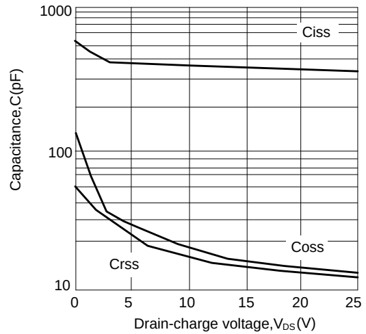
Figure 4: Capacitance characteristics
