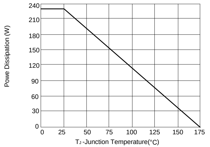
Figure 8: Power De-rating
