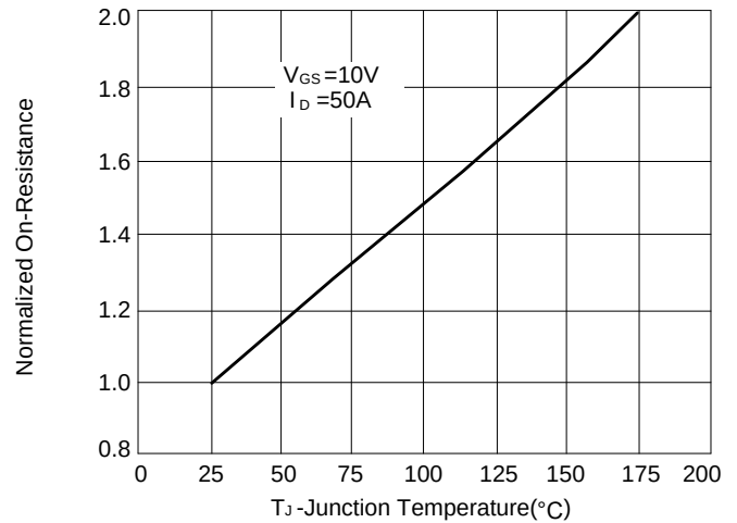
Figure 2: Rdson-Junction Temperature
