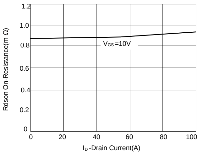
Figure 5: Rdson-Drain Current
