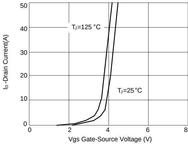
Figure 3: Transfert Characteristics
