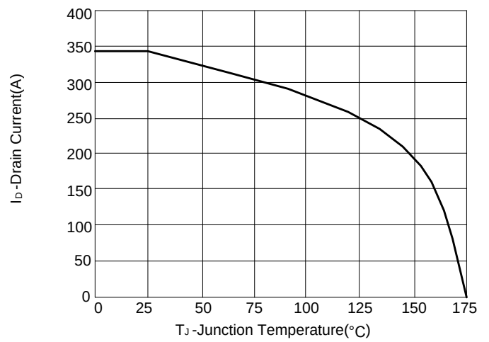
Figure 10: Current De-tating
