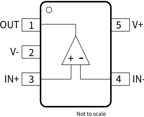
Figure 1-1 NSOPA9011 5-Pin SOT-23 Package Top View
