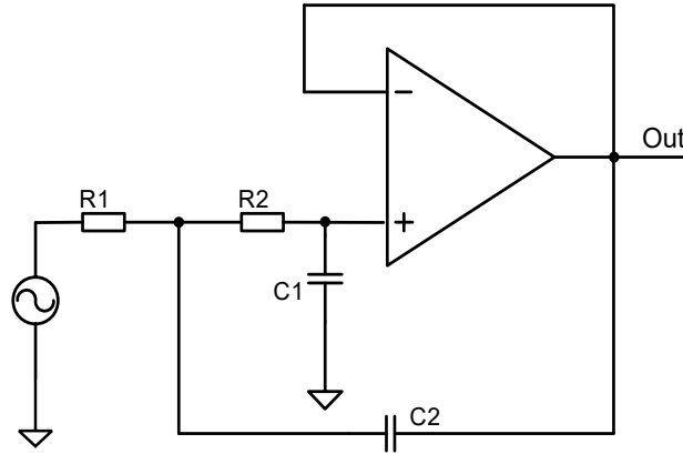
Figure 9-1 2nd order Sallen-key filter
