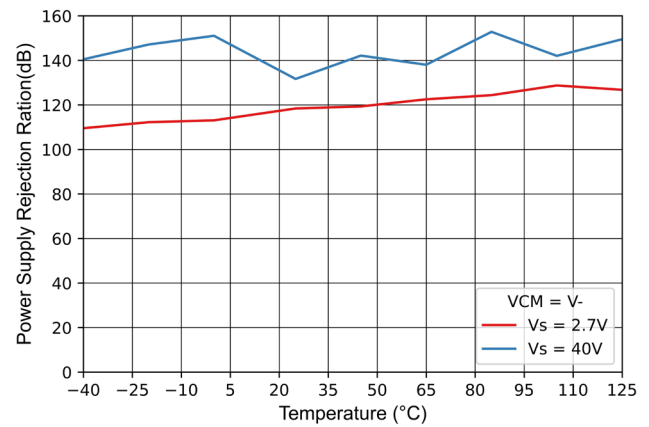
Figure 7-8 PSRR vs Temperature
