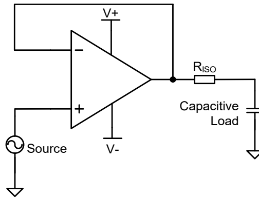
Figure 8-8 Insert isolation Resistor to drive large Capacitive Load
