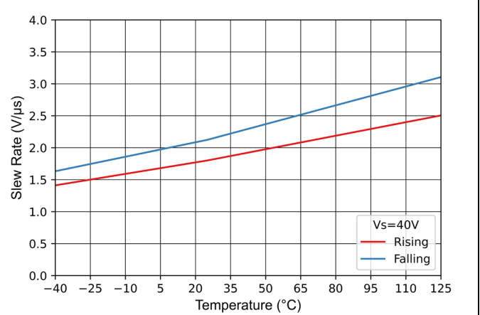
Figure 7-22 Slew Rate vs Temperature
