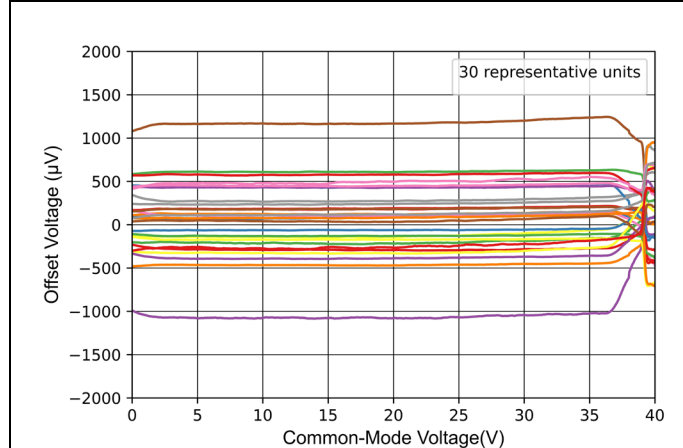
Figure 7-3 Offset Voltage vs Common-Mode Voltage
