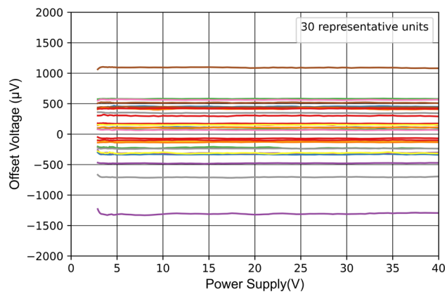
Figure 7-7 Offset Voltage vs Power Supply ( V_{CM} = V_- )
