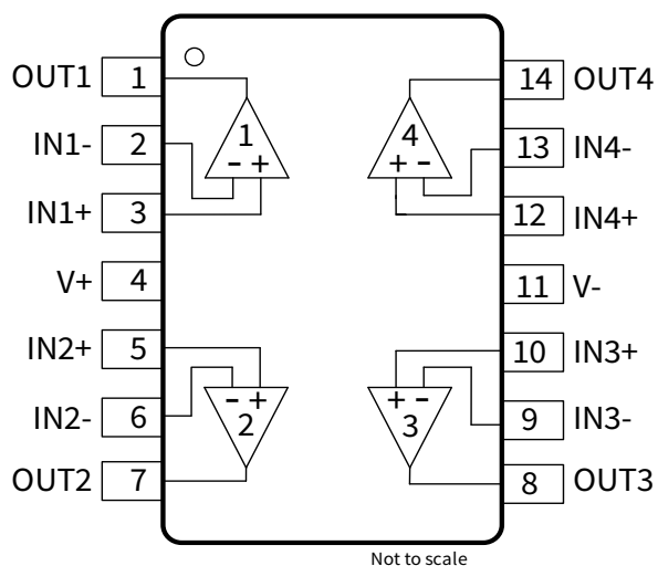
Figure 1-4 NSOPA9014 14-Pin SOP and TSSOP Package Top View
