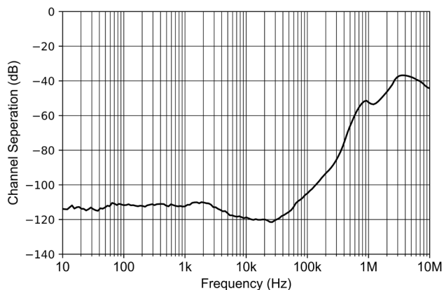
Figure 7-37 Channel Separation vs Frequency
