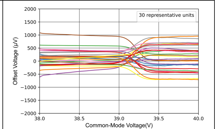
Figure 7-4 Offset Voltage vs Common-Mode Voltage, Transition
