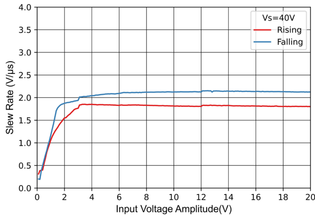
Figure 8-4 Slew-Rate vs Input Voltage Amplitude
