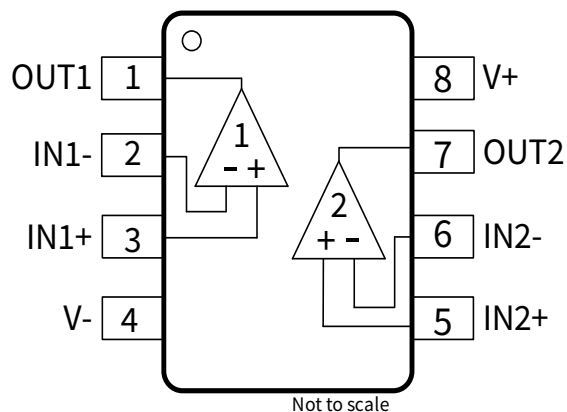
Figure 1-3 NSOPA9012 8-Pin SOP and MSOP Package Top View
