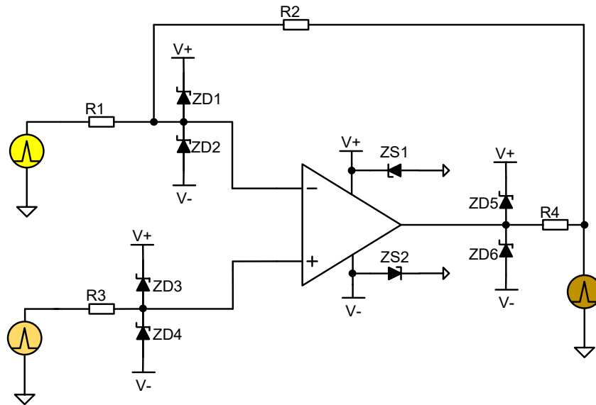
Figure 8-11 External component to enhance EOS performance
