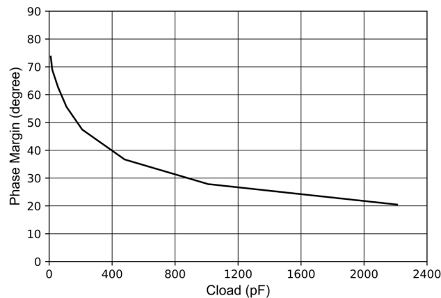
Figure 8-7 NSOPA901x Phase Margin vs Capacitive Load
