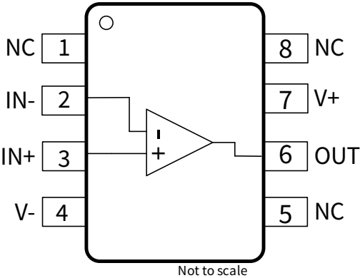
Figure 1-2 NSOPA9011 8-Pin SOP Package Top View
