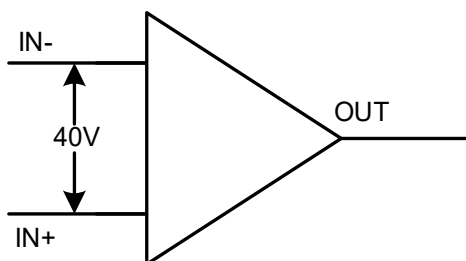
Figure 8-2 NSOPA901x input stage
