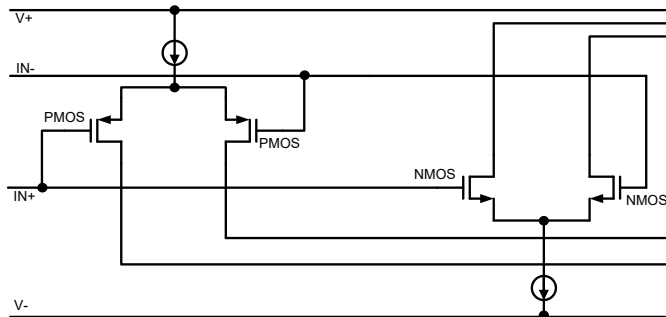
Figure 8-5 NSOPA901x Rail-to-rail Input Stage
