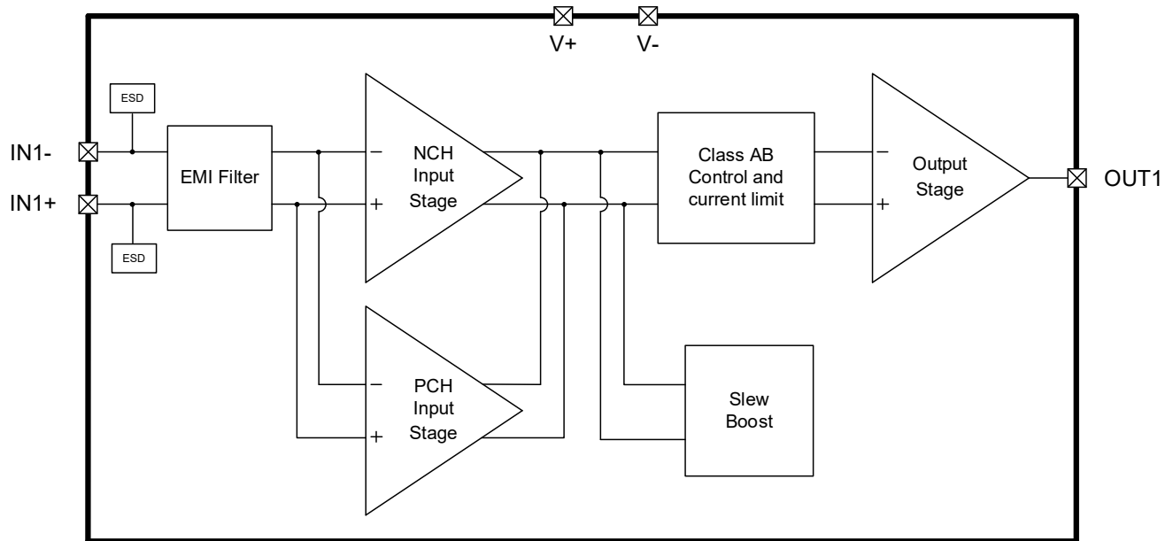
Figure 8-1 NSOPA901x Functional block Diagram (One channel is shown)
