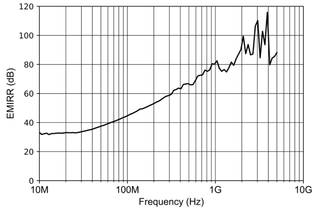
Figure 8-6 NSOPA901x EMIRR vs Frequency
