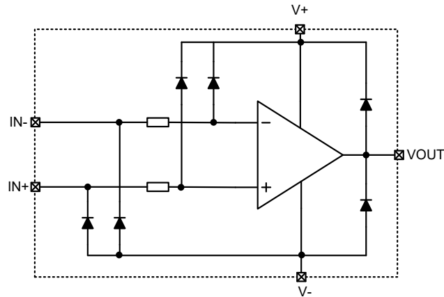
Figure 8-10 Internal ESD Equipment Model
