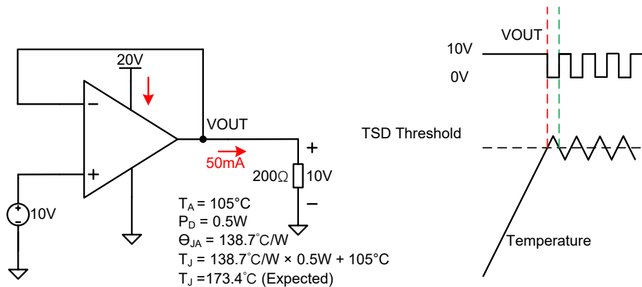
Figure 8-9 Thermal shut down and recovery
