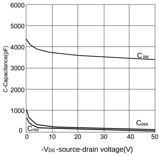
Figure 9 Capacitance
