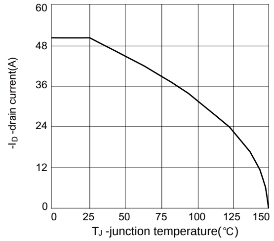
Figure 2 Current capability
