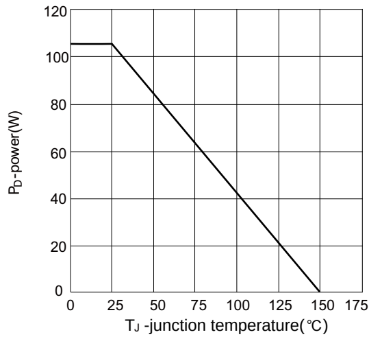
Figure 1 Power capability
