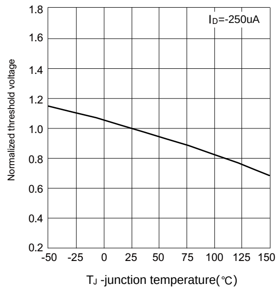
Figure 6 Normalized threshold voltage
