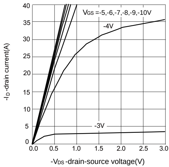
Figure 3 Output characteristics
