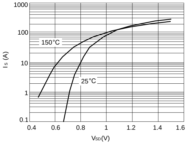
Figure 7: Body Diode Forward Characteristics
