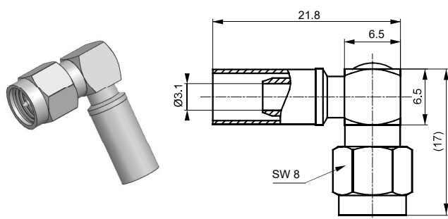
SMA-JW5AY
