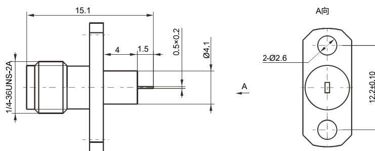
SMA-KFD-206
