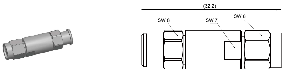
SMA-J480BG
