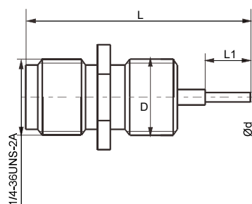
SMA-KYD-11
