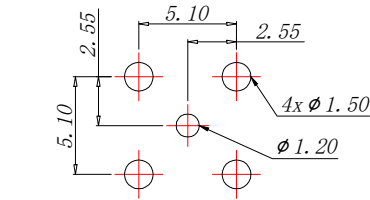
PCB WELDING DRAWING (TOLERANCE: ±0.05)
