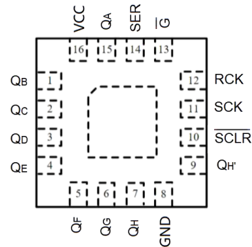
QFN-16
