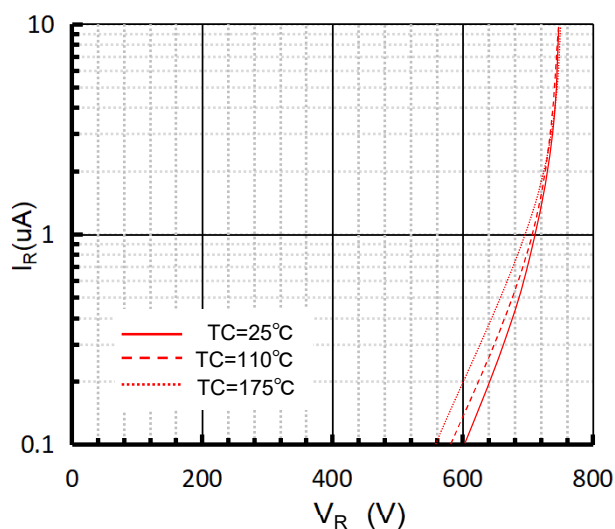
Fig 4. Reverse Characteristics
