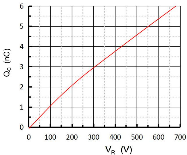
Fig 6. Reverse Charge vs. Reverse Voltage
