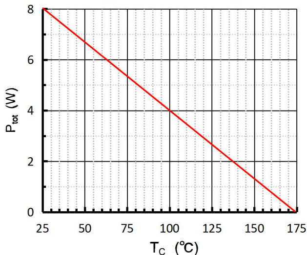
Fig 2. Power Derating
