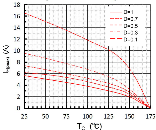
Fig 1. Current Derating
