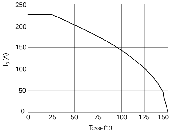
Figure 7:current de-rating
