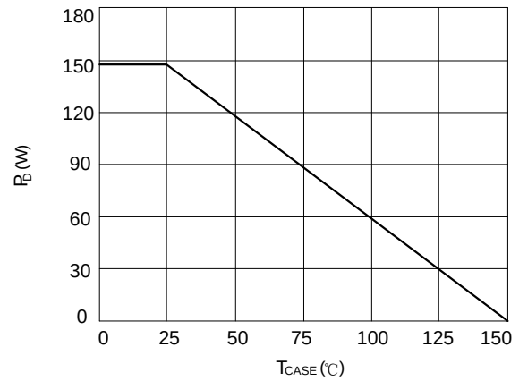
Figure 8:power de-rating
