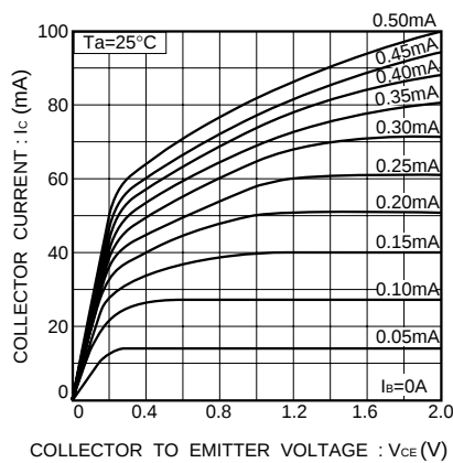
Fig.2 Grounded emitter output characteristics ( I )
