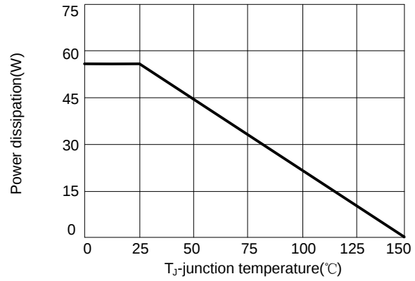
Figure 8 :Power de-rating
