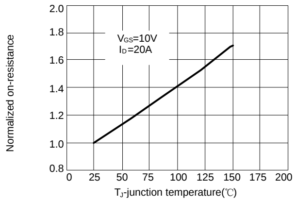
Figure 2 :Rdson-junction temperature
