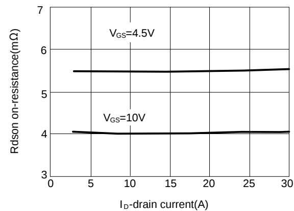
Figure 5 :Rdson-drain current
