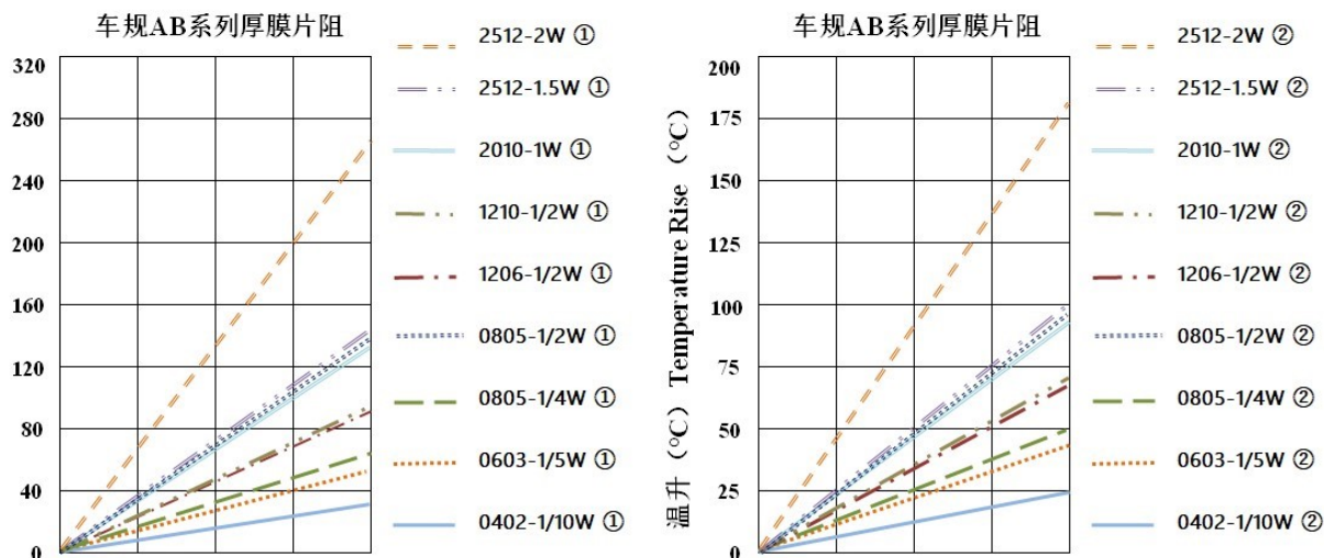
Thick Film Chip Fixed Resistor Automotive Grade (AB series)
