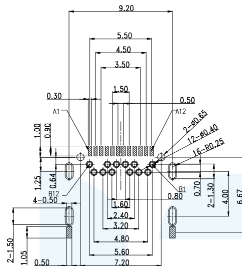
RECOMMENDED P.C.B LAYOUT(COMPANENT SIDE)
