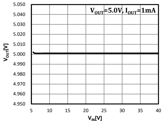
Figure 6. Line Regulation vs V_{IN}
