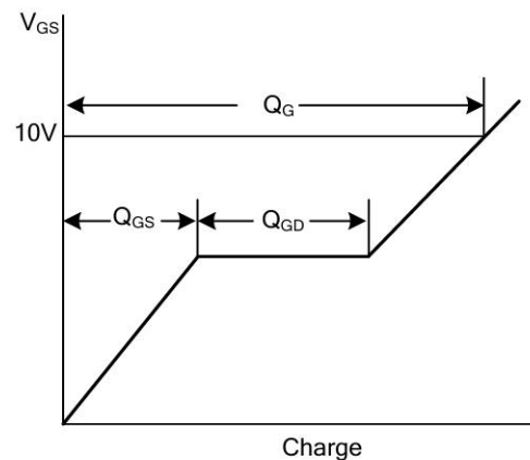
Gate Charge Waveforms
