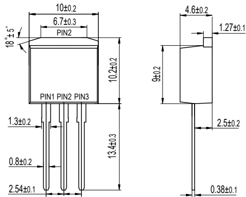
TO-262AB MURW20XX
