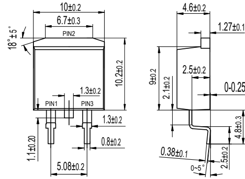
TO-263(D 2 PAK) MURD20XX
