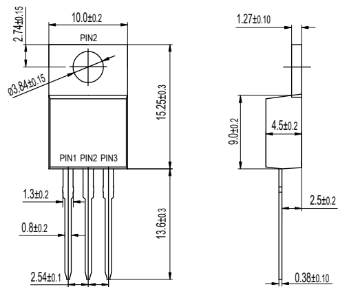
TO-220AB MUR20XX
