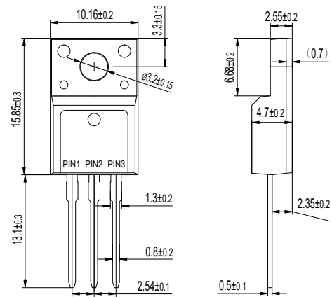
ITO-220AB MURF20XX
