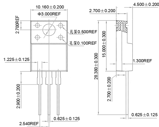
ITO-220AB MURF10XXCT
