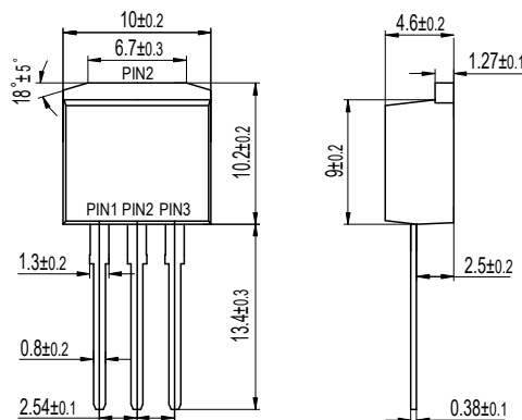
TO-262AB MURW10XXCT
