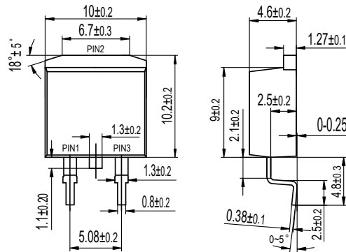
TO-263(D 2 PAK) MURD10XXCT
