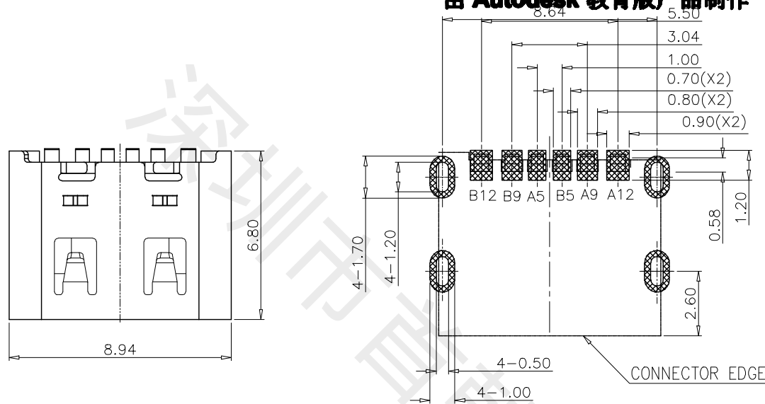
RECOMMENDED PCB LAYOUT(TOP VIEW) THICKNESS 1.6 \pm 0.10\text{MM} ; DEFAULT TOLERANCE: \pm 0.05
