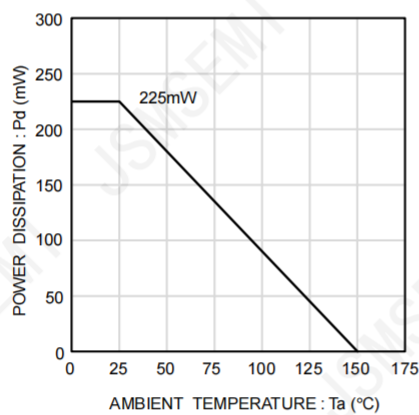
Fig.2 Derating curve
