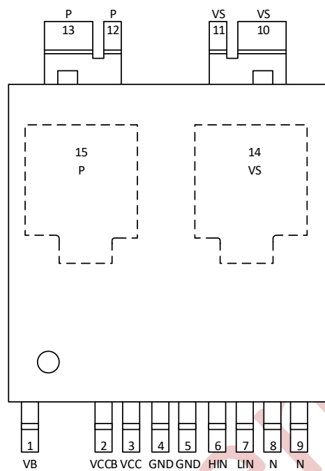
Fig2 Footprint Description
