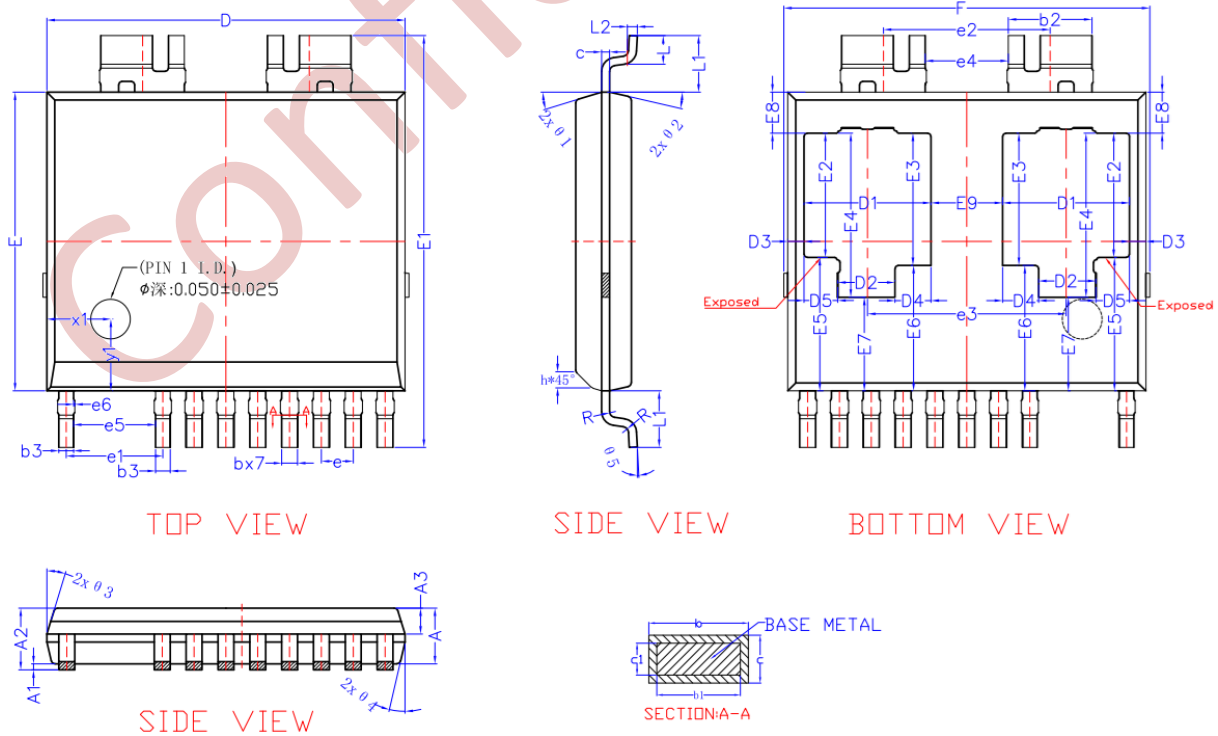
Package Outlines
