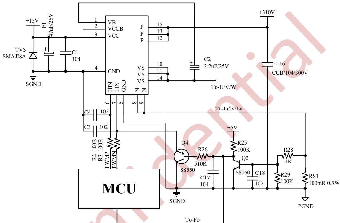
Fig.6 Typical Application Connection NSH305M0PC
