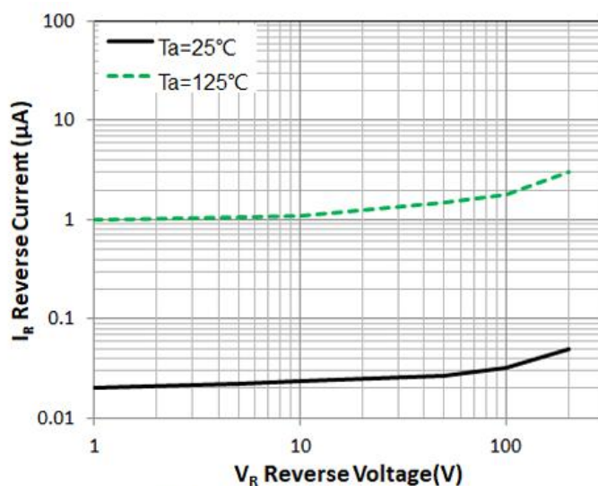
Figure 2. Reverse Characteristic(typ.)
