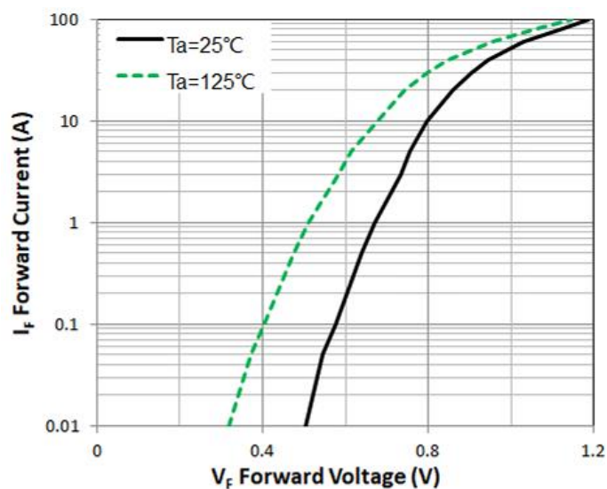
Figure 1. Forward Characteristic(typ.)
