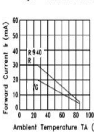
Fig.3 FORWARD CURRENT DERATING CURVE
