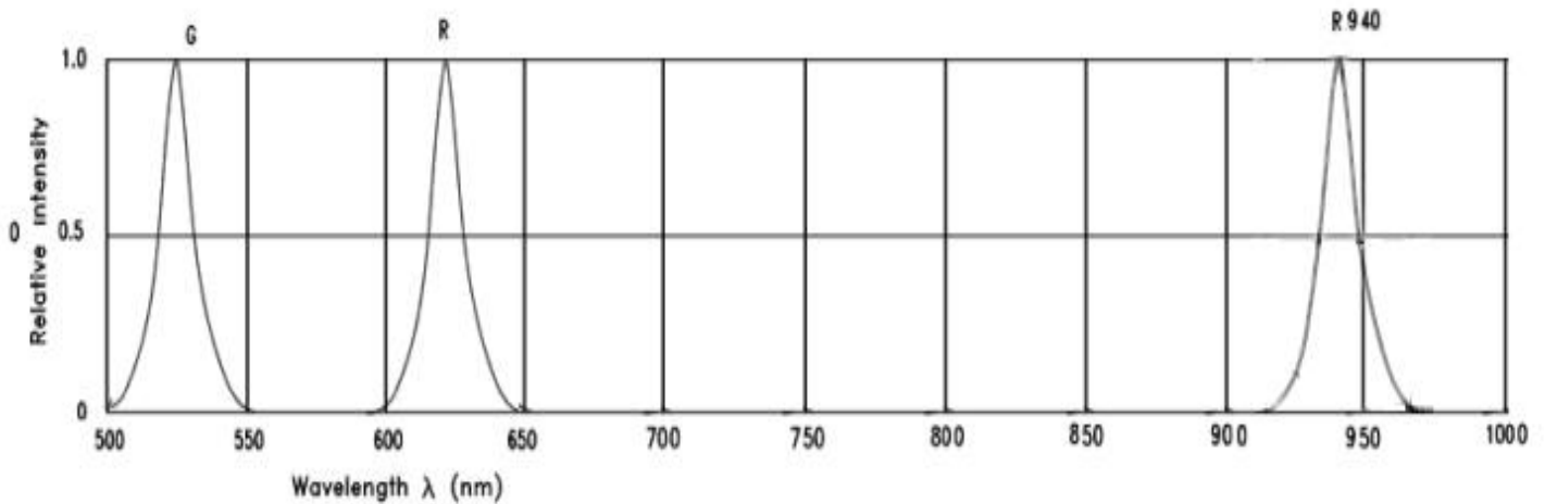
Fig.1 RELATIVE INTENSITY VS. WAVELENGTH
