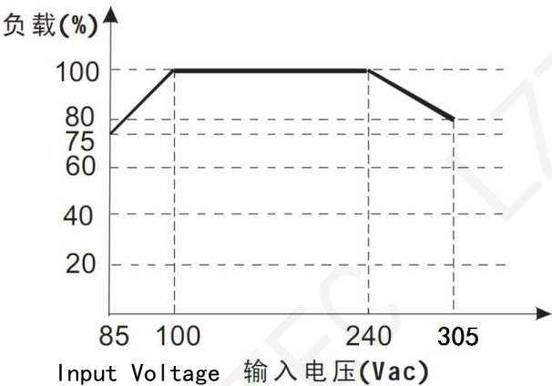
Input Voltage vs. Load Correlation
