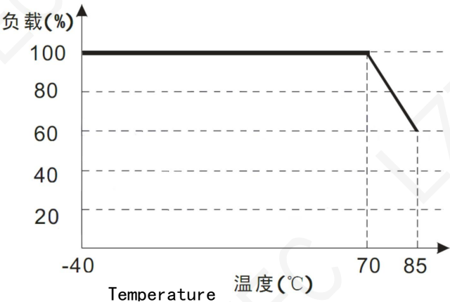
Temperature vs. Load Correlation
