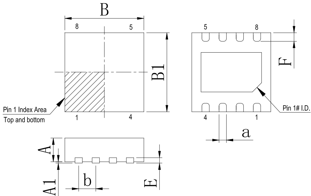
Dimensions In Millimeters(DFN-8 3*3)
