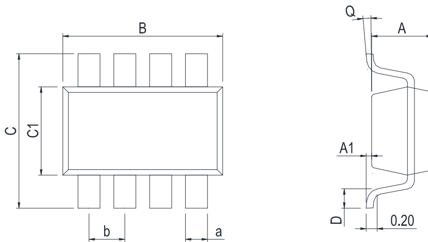
Dimensions In Millimeters(SOT-23-8)
