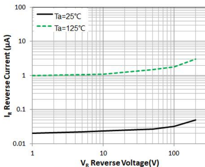
Figure 2. Reverse Characteristic(typ.)
