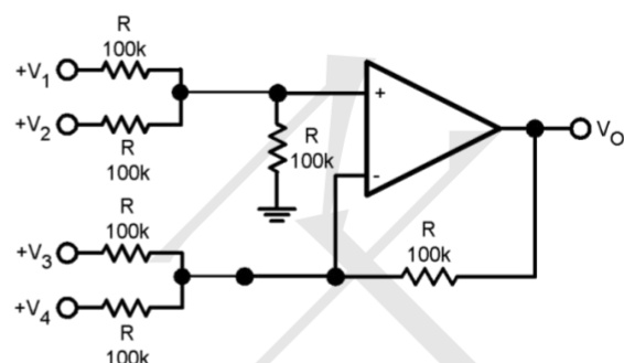
DC adder amplifier
