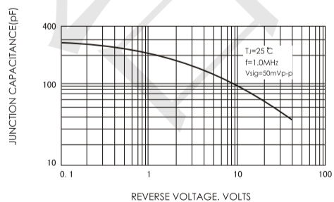
FIG.5-TYPICAL JUNCTION CAPACITANCE
