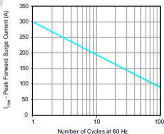
Maximum Non-Repetitive Forward Surge Current Uni-Directional Only
