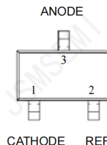
N Package (SOT-23)
