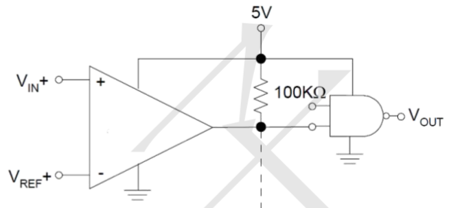
Driving CMOS
