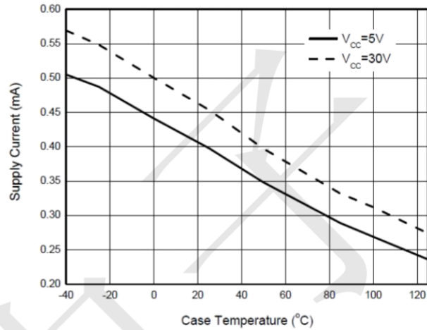
Fig. 2 Supply Current vs. Case Temperature
