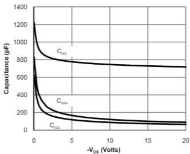
Figure 7: Capacitance Characteristics
