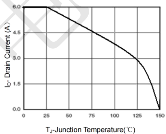
Figure 4 Drain Current
