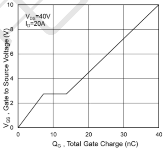
Fig.4 Gate to Source Voltage vs Total Gate Charge
