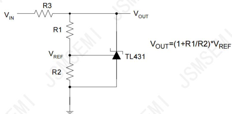
Figure 17. Shunt Regulator
