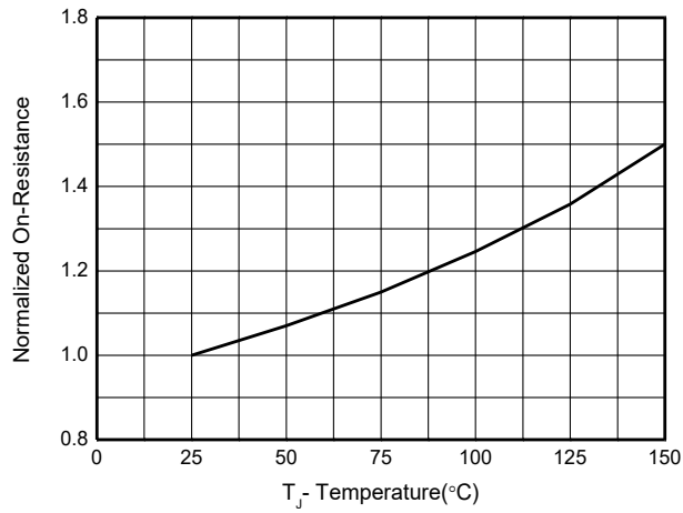
Figure 7. Rdson-Junction Temperature(°C)
