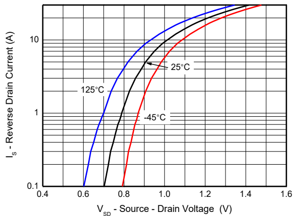
Figure 5. Body-Diode Characteristics
