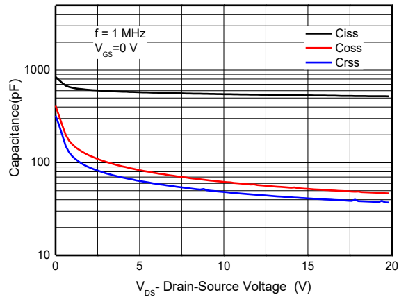
Figure 3. Capacitance Characteristics
