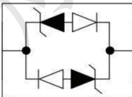
DFN1006-2
