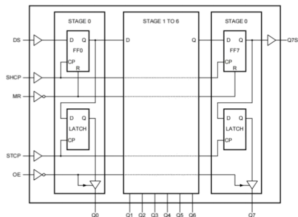
Figure 3. Logic diagram
