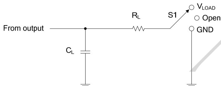
TEST CIRCUIT
