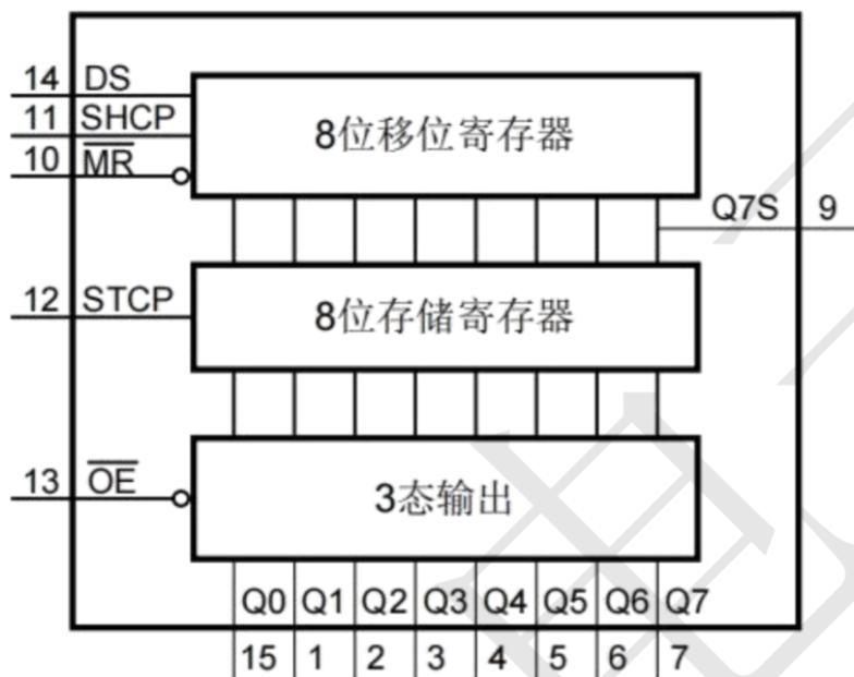
Figure 4. Functional diagram
