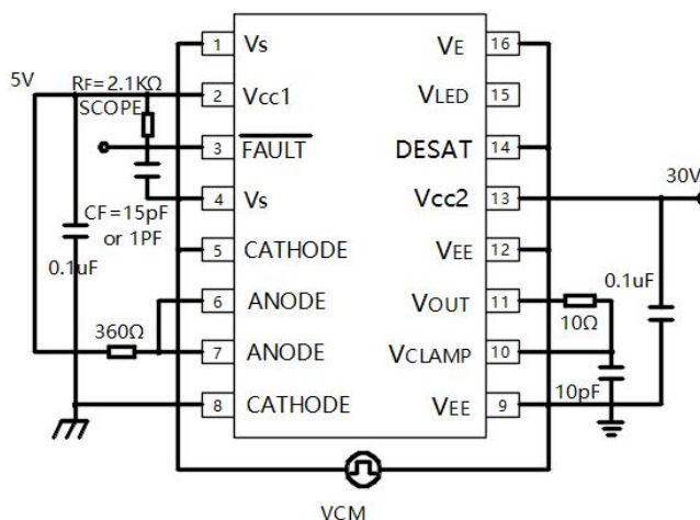
Fig32. CMR Test Circuit LED2 on
