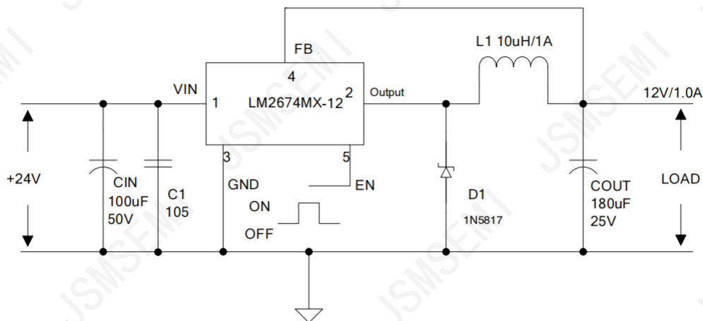
LM2674MX-12 System Parameters Test Circuit
